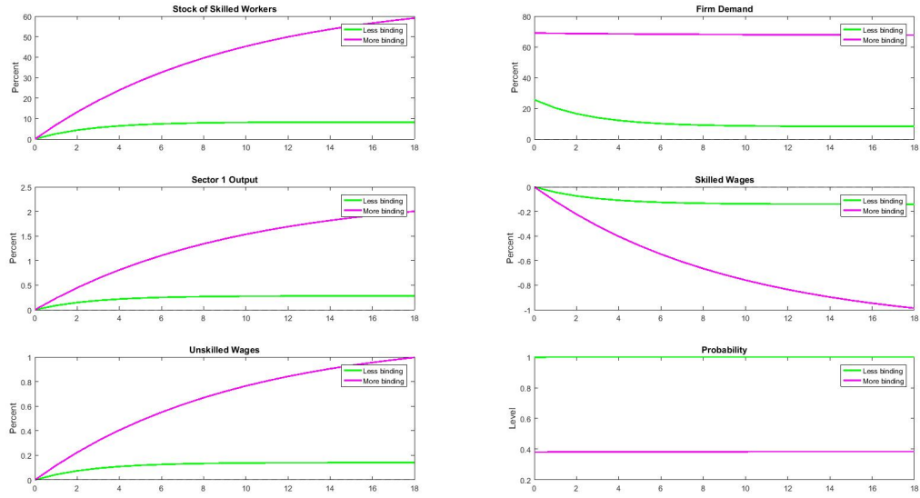
Figure 5: Transitional dynamics after a 10 percent cap change when the cap is ‘more binding’ vs the case when it is ‘less binding’. All variables (except probability) are in percent deviation from the steady state.
