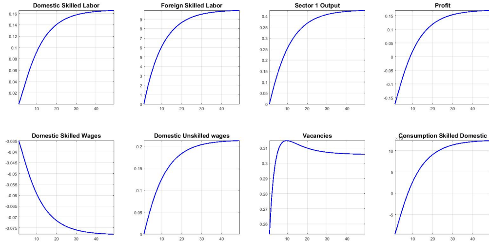
Figure 6: Transition dynamics after a 10 percent cap change in the search and matching model. All variables are in percent deviation from the steady state.
