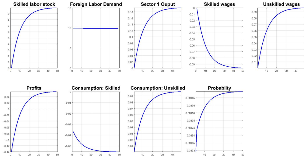
Figure 4: Transitional dynamics after a 10 percent increase in the skilled immigration cap. All variables (except probability) are in percent deviation from the steady state.
